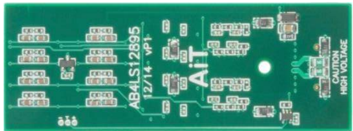
Back view
